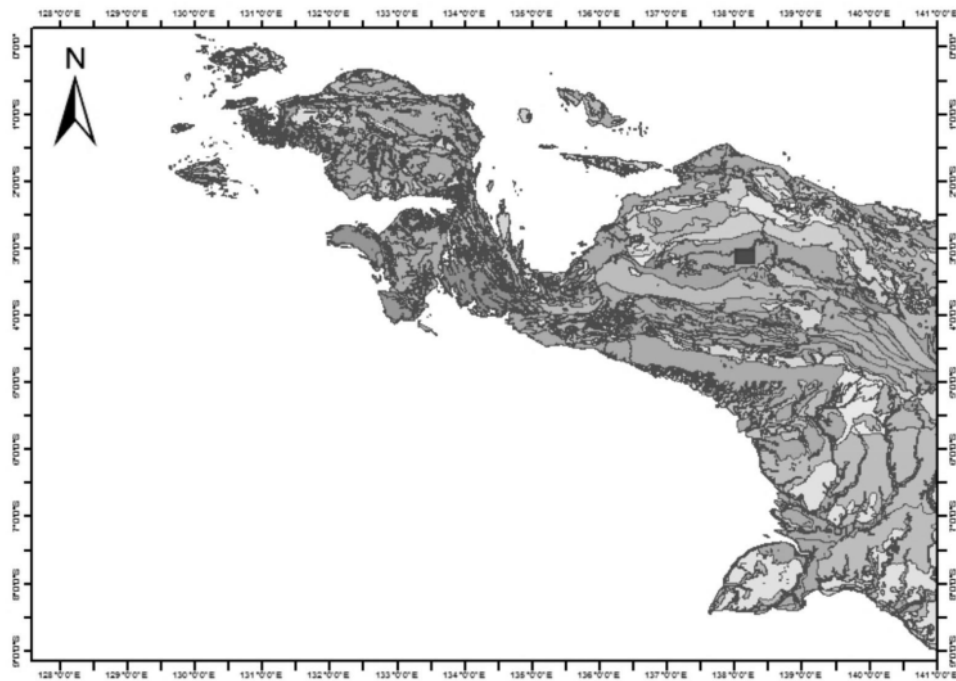
2 Fig. 1. Regional geological map of Papua (after Dow and Sukanto, 1984) and the research area (not to scale).
